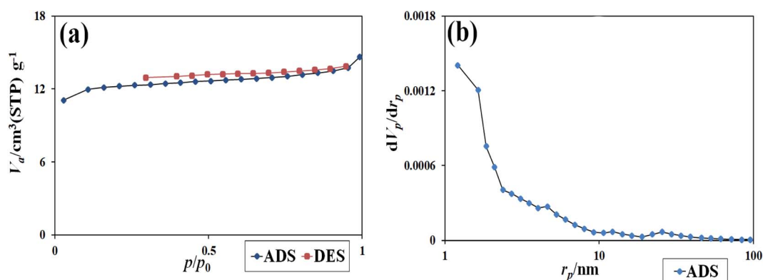
Fig. 11 (a) The isotherm obtained from the study of \text{N}_2 adsorption/desorption on \text{Ti}_4\text{HgI}_6/\text{HgI}_2 nanocomposite, (b) the graph obtained from BJH calculations of sample no. 8.
