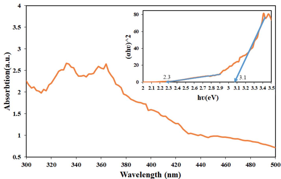
Fig. 10 DRS analyses from sample no. 8 as the optimal sample and inset resulting graph to estimate the band-gap of \text{Ti}_4\text{HgI}_6/\text{HgI}_2 nanocomposite.
