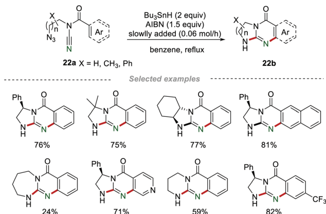
Scheme 22 The construction of guanidines.
