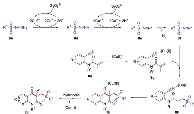
Scheme 8 The construction of sulfonylated quinoline-2,4-diones.
