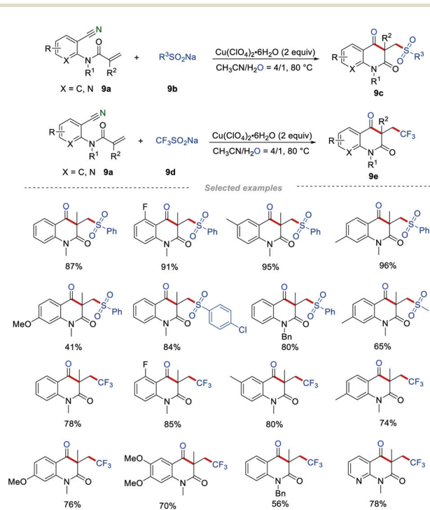
Scheme 9 The construction of sulfonylated and trifluoromethylated quinoline-2,4-diones.
