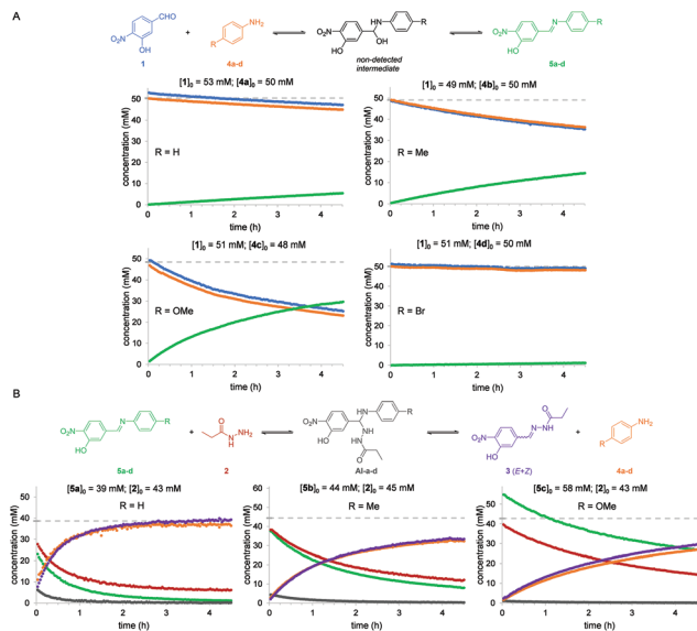
Fig. 3 (A) Reaction between aldehyde 1 and anilines 4a–d in CD 3 CN to form imines 5a–d. Plots show the concentrations (mM) of compounds 1, 4a–d and 5a–d at different reaction times using approximately equal initial concentrations of reagents 1 and 4a–d. Grey dashed lines indicate the initial concentrations of the limiting reagents for each reaction. (B) Reaction between imines 5a–d and acylhydrazide 2 in CD 3 CN to form acylhydrazone 3 as a mixture of Z/E isomers. Plots show the concentrations (mM) of compounds 4a–c, 3 and 5a–c at different reaction times using approximately equal initial concentrations of reagents 5a–c and 3. Grey dashed lines indicate the initial concentrations of the limiting reagents for each reaction. Imine 5d was discarded due to its poor solubility in CD 3 CN at the concentrations required for NMR analysis.
