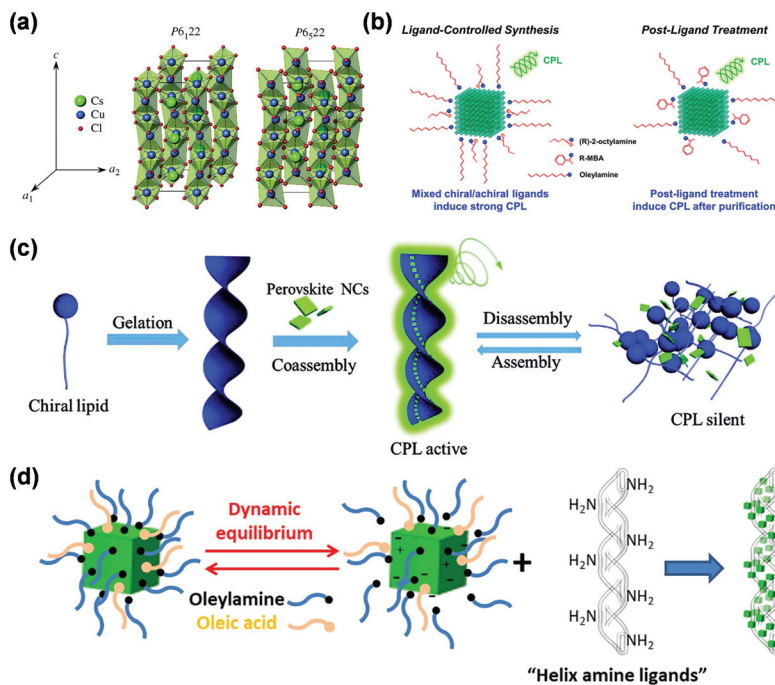
Fig. 3 (a) Schematic illustration of enantiomorphic crystal structures of \text{CsCuCl}_3 . This figure has been adapted/reproduced from ref. 87 with permission from Wiley-VCH, Copyright 2013. (b) The post-treatment induced chirality in perovskite NCs by ligand exchange with chiral organic molecules. This figure has been adapted/reproduced from ref. 90 with permission from American Chemical Society, Copyright 2020. (c) Schematic illustration of assembly-induced chirality in perovskite NCs by chiral gels. This figure has been adapted/reproduced from ref. 93 with permission from Wiley-VCH, Copyright 2018. (d) Schematic illustration of the synthesis of chiral helical \text{CsPbBr}_3 NCs arranged on inorganic silica nanohelices. This figure has been adapted/reproduced from ref. 97 with permission from American Chemical Society, Copyright 2020.
