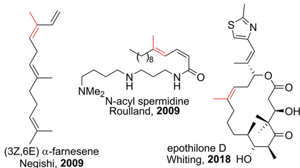
Scheme 24 Select natural products synthesised via haloboration/cross-coupling sequences. The fragment incorporated in such manner is coloured in red.
