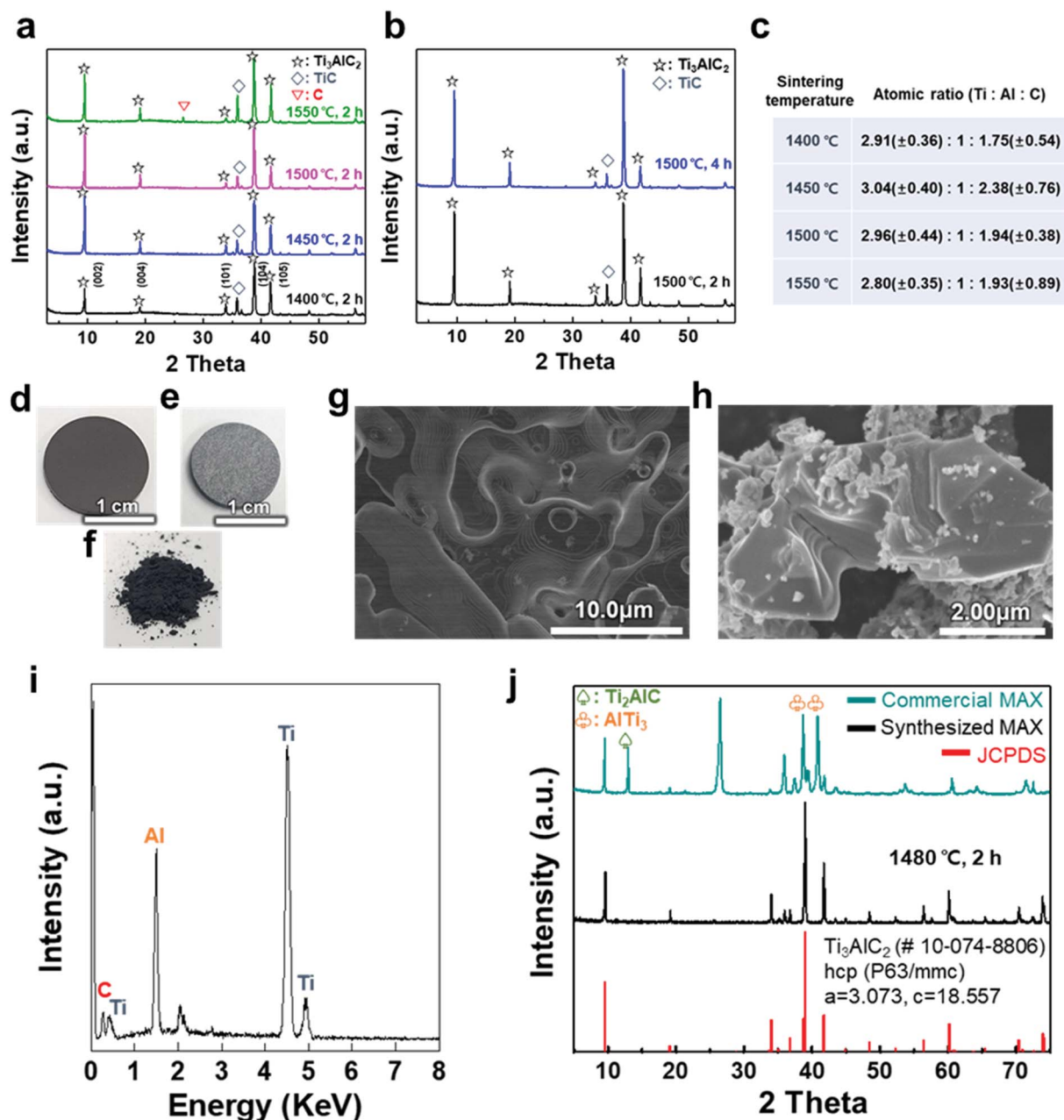
Fig. 1 (a) XRD patterns of as-milled \text{Ti}_3\text{AlC}_2 MAX phase pellets sintered at various sintering temperatures, (b) XRD patterns of the pellets sintered at 1500 °C at different times, and (c) calculated atomic ratio based on sintering temperature. Photographs of a cold-pressed pellet (d) before and (e) after the sintering process at \approx 1480 °C for 2 h, and (f) as-milled powder. SEM images of the (g) sintered pellet surface and (h) as-synthesized MAX phase with a layered structure after grinding. (i) EDX spectrum of a pellet, revealing the chemical composition of the \text{Ti}_3\text{AlC}_2 MAX phase, and (j) XRD patterns of commercial and as-synthesized \text{Ti}_3\text{AlC}_2 MAX phase powder compared with hexagonal closed-packed \text{Ti}_3\text{AlC}_2 (JCPDS 10-074-8806).
