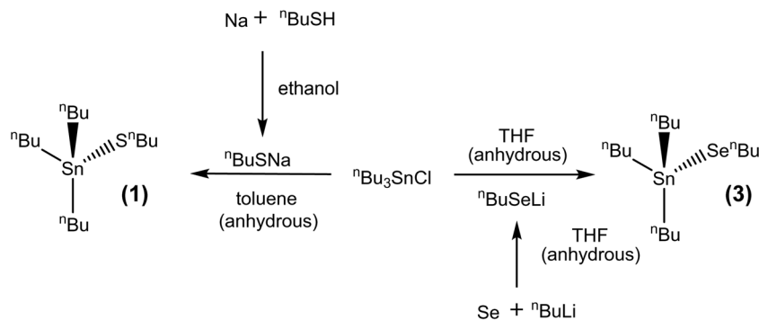
Scheme 1 Synthesis of [Sn n Bu 3 (E n Bu)] (E = S, Se) (1) and (3).
