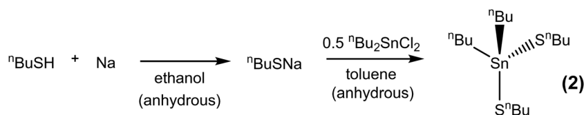
Scheme 2 Synthesis of [Sn n Bu 2 (S n Bu) 2 ] (2).
