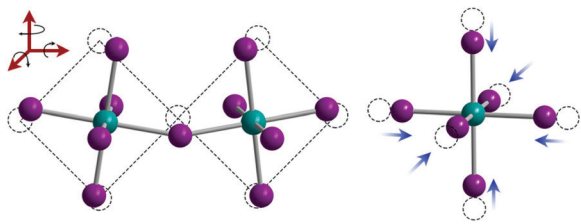
Fig. 10 Pressure-induced rotation of \text{PbI}_6 octahedra (left) and \text{Pb-I} bond compression (right). Reproduced with permission from ref. 160. Copyright 2017, American Chemical Society.
