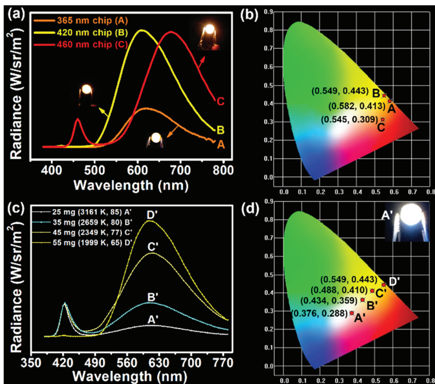
Fig. 4 (a) EL spectra and (b) CIE coordinates of LEDs based on different kinds of chips combined with CPDs under 3.0 V. (c) EL spectra and (d) CIE coordinates of the LEDs based on different amounts of CPDs combined with a 420 nm blue chip under 3.0 V. The insets are corresponding digital photographs.
