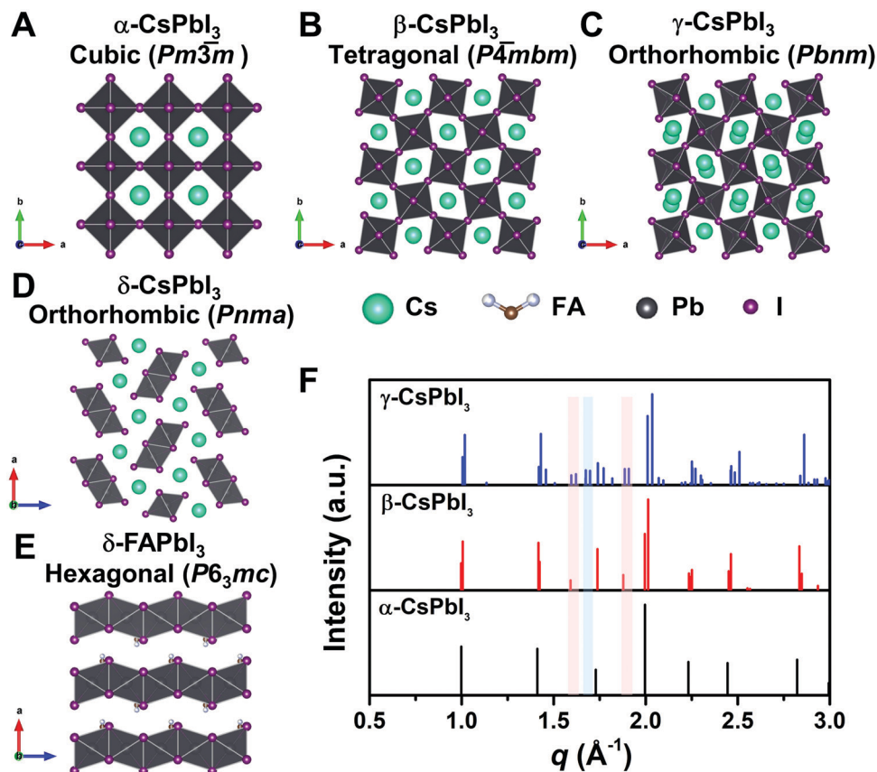
Fig. 3 Crystal structure of three perovskite phases with corner-sharing octahedra for CsPbI 3 , which are cubic α-CsPbI 3 (A), tetragonal β-CsPbI 3 (B), and orthorhombic γ-CsPbI 3 (C). (D) and (E) show the crystal structure of non-perovskite δ-CsPbI 3 and δ-FAPbI 3 , respectively. All the crystal structures in A–E were plotted via Vesta using crystallographic information files extracting from ref. 25, 44 and 45. (F) Simulated powder XRD patterns for the α-, β-, and γ-phases of CsPbI 3 plotted with vertical lines corresponding to the diffraction peaks. XRD patterns plotted with respect to the scattering vector q , which is equivalent to 2 \times \pi/d where d is the d -spacing of the diffracting set of planes. The red-shaded areas show the positions of the extra XRD peaks discussed in the main text for tetragonal and orthorhombic structures compared with the cubic structure. The blue-shaded area exhibits the position of the additional XRD peak discussed in the main text for orthorhombic structures compared with the cubic and tetragonal structures. XRD patterns were simulated using Vesta.
