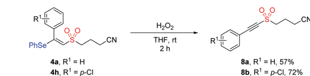
Scheme 2 Synthetic application.
