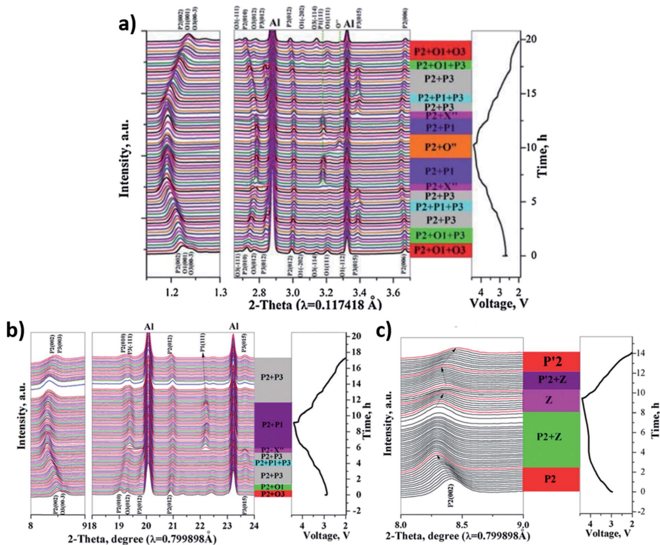
Fig. 16 In operando XRD data for (a) P2/O1/O3 (b) P2/O3 (c) P2-Na x Ni x Ni 1/3 Co 1/3 Mn 1/3 O 2 cycling between 2.0–4.4 V at 0.1C together with their phase evolution. Reproduced from ref. 164 with permission from The Royal Society of Chemistry.
