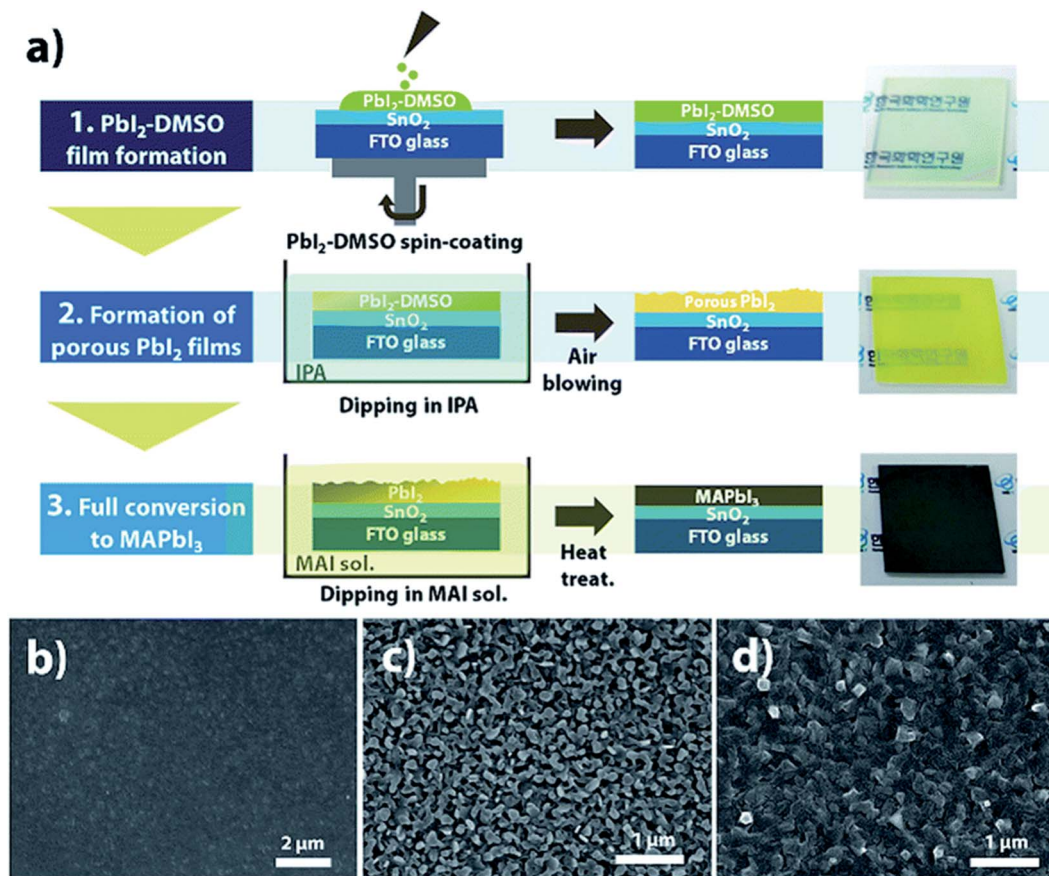
Fig. 19 (a) Schematic diagram of mediator extraction treatment (MET) representing each step and optical images of the resulting perovskite films. The scanning electron microscope images of (b) Pbl 2 -DMSO, (c) Pbl 2 , and (d) MAPbl 3 films fabricated by MET. Reproduced by permission ref. 130, Copyright 2018 Royal Society of Chemistry.
