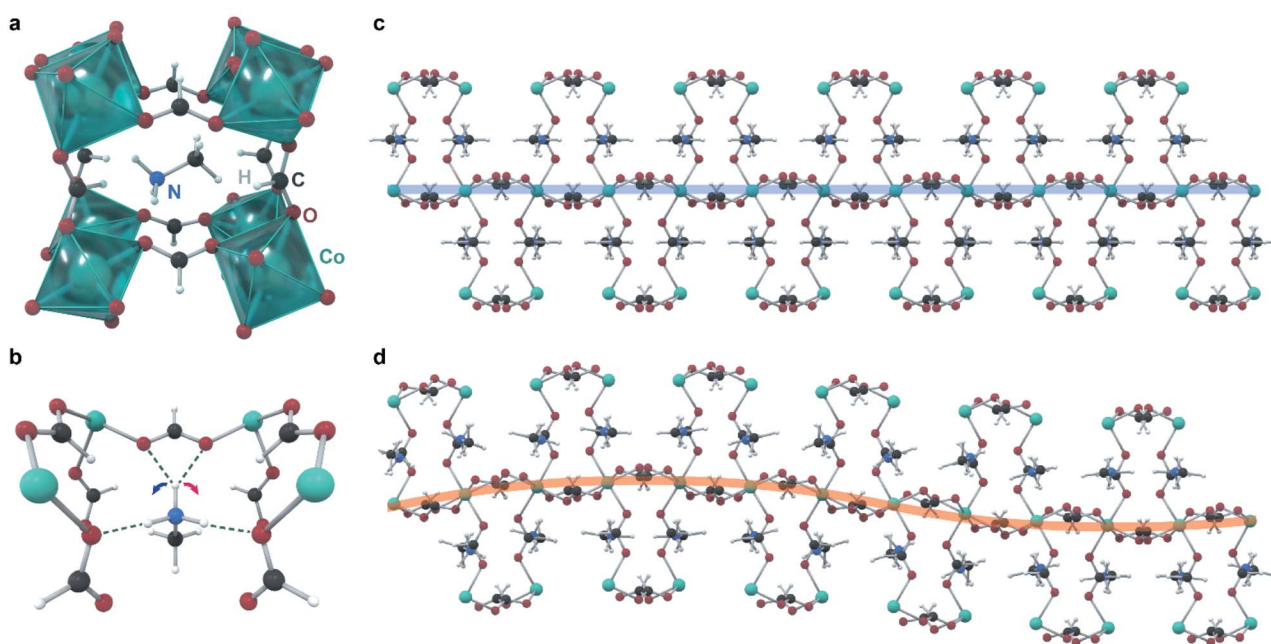
Fig. 4 Structure of the incommensurate modulation in the perovskitic cobalt formate. (a) Each unit cell of the average structure contains one methylammonium cation in a perovskite cage of cobalt formate. (b) The methylammonium cation has close contacts with four formate oxygens, with mirror symmetry; in the modulated structure this symmetry is broken. (c) Structure of the commensurate phase, given for comparison. (d) A supercell depicting the modulation vector (amplitude of modulation scaled up six times for clarity).
