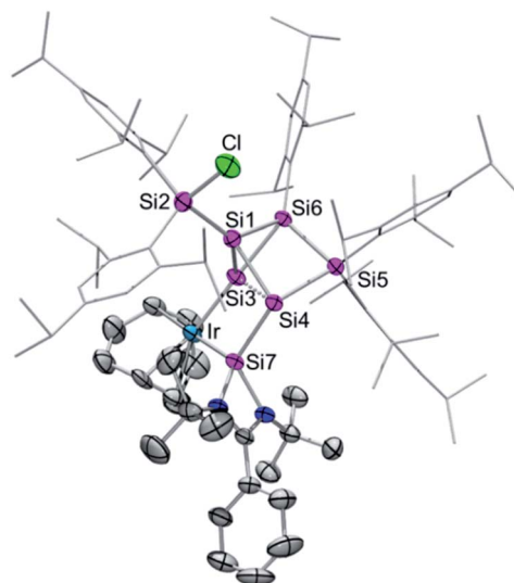
Fig. 1 Representative molecular structure of silylene-functionalized siliconoid iridium complex 2a in the solid state. Hydrogen atoms are omitted for clarity. Thermal ellipsoids are set at 50% probability. For structures of 2b,c see ESI†. Selected bond lengths [Å] and angles [°]: 2a : Ir–Si7 2.320(1), Ir–Si3 2.334(1), Si1–Si3 2.305(2), Si1–Si4 2.313(2), Si1–Si6 2.364(2), Si1–Si2 2.369(2), Si3–Si6 2.353(1), Si3–Si4 2.548(2), Si3–Si7 2.764(2), Si4–Si5 2.391(2), Si4–Si7 2.402(2), Si7–N2 1.857(3), Si7–N1 1.884(3), Cl–Si2–Si1 99.03(6), Si1–Si3–Ir 124.02(5), Ir–Si3–Si6 174.93(6), Ir–Si3–Si4 105.99(5), Ir–Si3–Si7 53.33(3), and Si7–Si4–Si3 67.81(4); 2b : Ir–Si3 2.3517(7), Ir–Ge 2.4113(3), Ge–Si4 2.4444(8), Ge–Si3 2.8481(8), Si1–Si3 2.296(1), Si1–Si4 2.302(1), Si1–Si2 2.356(1), Si1–Si6 2.375(1), Si3–Si6 2.339(1), Si3–Si4 2.565(1), Si4–Si5 2.389(1), Si5–Si6 2.368(1), Ge–N2 1.995(2), Ge–N1 2.005(2), Cl–Si2–Si1 100.91(4), Ir–Si3–Ge 54.243(17), Ir–Si3–Si4 106.90(3), Si6–Si3–Ir 173.61(4), Si1–Si3–Ir 124.75(4), Ir–Ge–Si3 52.322(16), Ir–Ge–Si4 108.95(2), Si3–Ir–Ge 73.436(19), and Ge–Si4–Si3 69.25(3).
