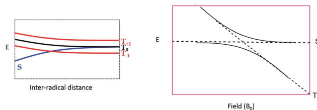
Fig. 7 The crossing region for S– T^- mixing. Left: S and T levels in an applied magnetic field, non-interacting. Right: expansion of the crossing region showing that some radical pairs will cross without interacting, but others will undergo an avoided crossing, and switch manifolds from T to S or vice versa.
