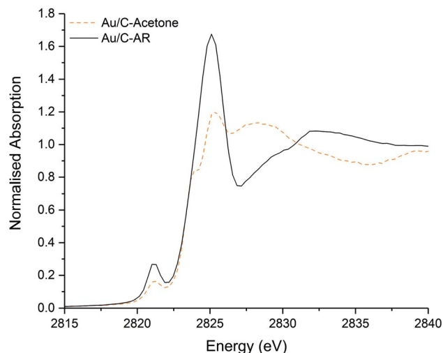
Fig. 4 Comparison of the normalised ex situ Cl K-edge XANES of the freshly prepared Au/C-acetone (dashed orange line) and Au/C-AR (black solid line).
