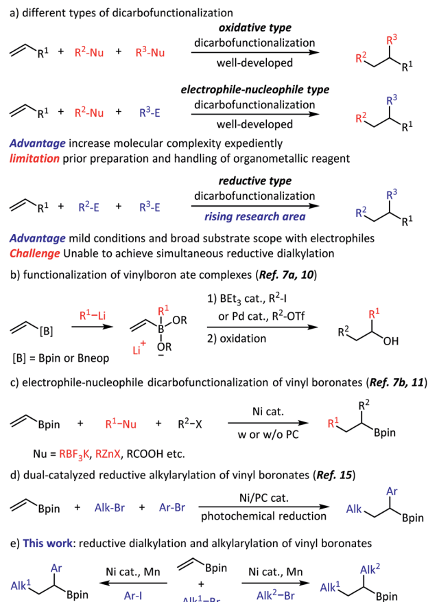
Scheme 1 Dicarbonylation of vinyl boronates to access alkylborates. B 2 pin 2 = bis(pinacolato)diboron. B 2 neop 2 = bis(neopentyl glycolato)diboron. Tf = triflyl. Nu = nucleophile. E = electrophile. w = with. w/o = without. PC = photoredox catalysis. Ar = aryl. Alk = alkyl.
