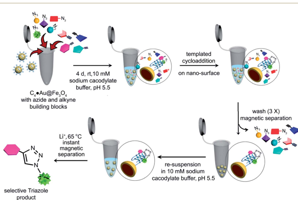
Fig. 4 Schematic representation of the target guided synthetic approach using i-motif magnetic nanotemplates ( c-MYC C 4 ·Au@Fe 3 O 4 & BCL2 C 4 ·Au@Fe 3 O 4 ) for in situ formation of potent binders.
