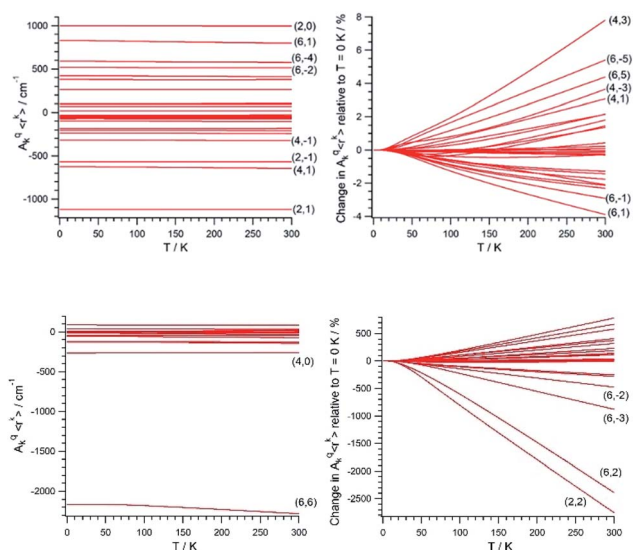
Fig. 2 Absolute (left) and relative to T = 0 \text{ K} (right) thermal evolution of the CFPs of [\text{U}(\text{Cp}^{\text{ttt}})_2]^+ (top) and \text{UTp}_3 (bottom). Some CFPs are identified as (k, q) , where k and q are the scripts k = 2, 4, 6 and q = -k, \dots, +k .
