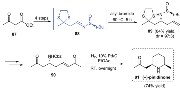
Scheme 16 Stereoselective synthetic protocol towards enantioenriched (-)-pinidinone.
