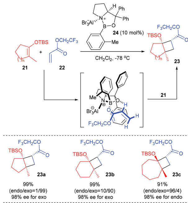
Scheme 7 [2 + 2] Cycloaddition of cyclic enolate silyl ether with propiolamide derivatives.
