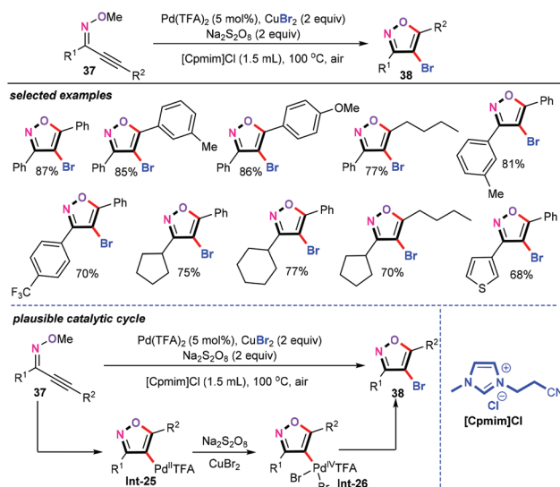
Scheme 18 Palladium-catalyzed cascade cyclization/bromination.
