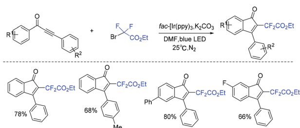
Scheme 61 The synthesis of difluoroacetylinidenones via the reaction of 1,3-diarylpropynones with ethyl bromodifluoroacetate.
