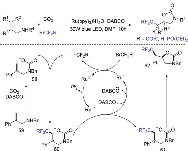
Scheme 34 The difluoroalkylation of allylamines with carbon dioxide.
