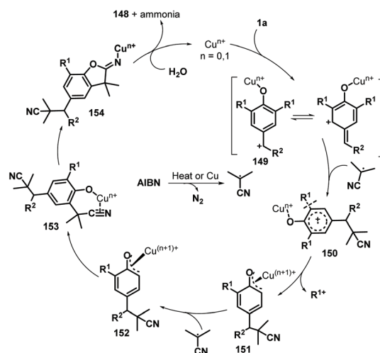
Scheme 31 Radical reaction of p -QMs with AIBN.
