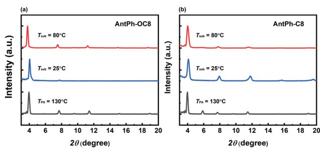
Fig. 4 XRD patterns of AntPh-OC8 (a) and AntPh-C8 (b) thin films prepared on OTS modified \text{SiO}_2/\text{Si} substrates at the various temperature conditions.
