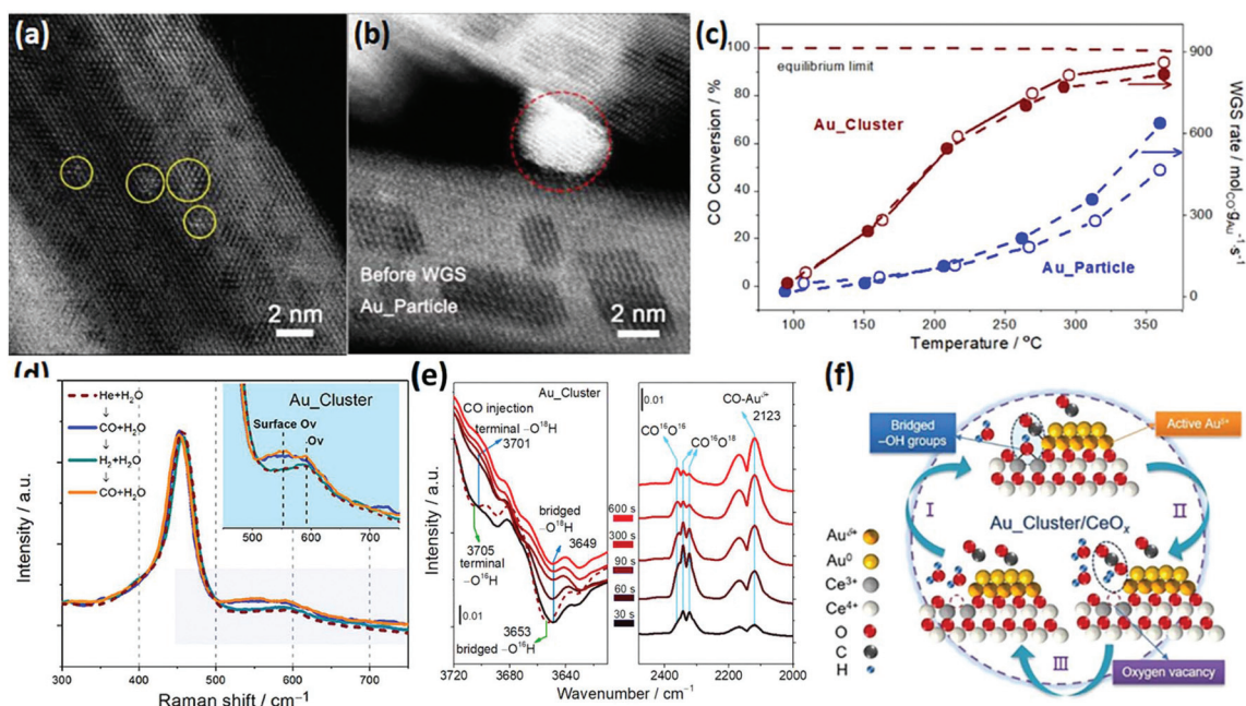
Fig. 14 High-angle annular dark-field scanning transmission electron microscopy (HAADF-STEM) images of (a) Au-cluster/ \text{CeO}_x and (b) Au-particle/ \text{CeO}_x catalyst. (c) Catalytic activity for the WGS by the Au-cluster/ \text{CeO}_x and Au-particle/ \text{CeO}_x catalysts. (d) In situ Raman spectra of Au-cluster/ \text{CeO}_x under different atmospheres at 150 °C. (e) In situ time-sequencing IR spectra of Au-cluster/ \text{CeO}_x under CO injection with isotope prelabeling using \text{H}_2\text{O}^{18} . (f) Schematic illustration of the reaction mechanism of Au-cluster/ \text{CeO}_x catalyst for the WGS. Adapted with permission from ref. 15. Copyright 2019, American Chemical Society.
