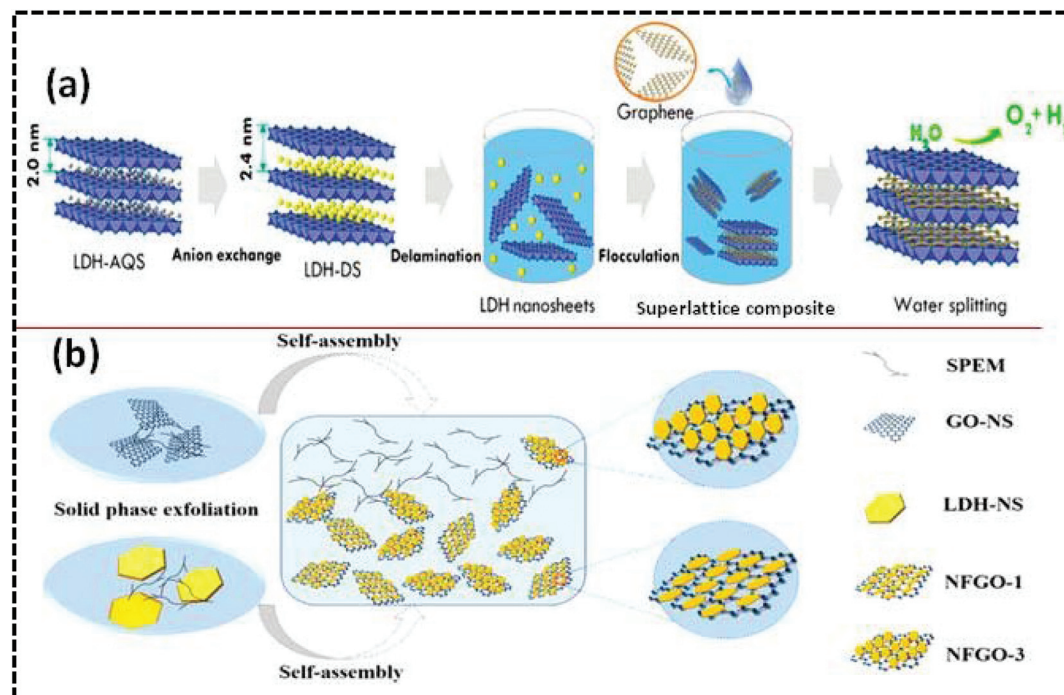
Fig. 9 (a) Illustration of the heterostructure formation of NiFe-LDH NS and graphene for water splitting. Reproduced with permission from ref. 83, Copyright 2015, American Chemical Society. (b) Synthetic steps of NiFe-LDH/GO nano hybrids by using the solid-phase exfoliation-liquid-phase assembly strategy. Reproduced with permission from ref. 73, Copyright 2019, American Chemical Society.
