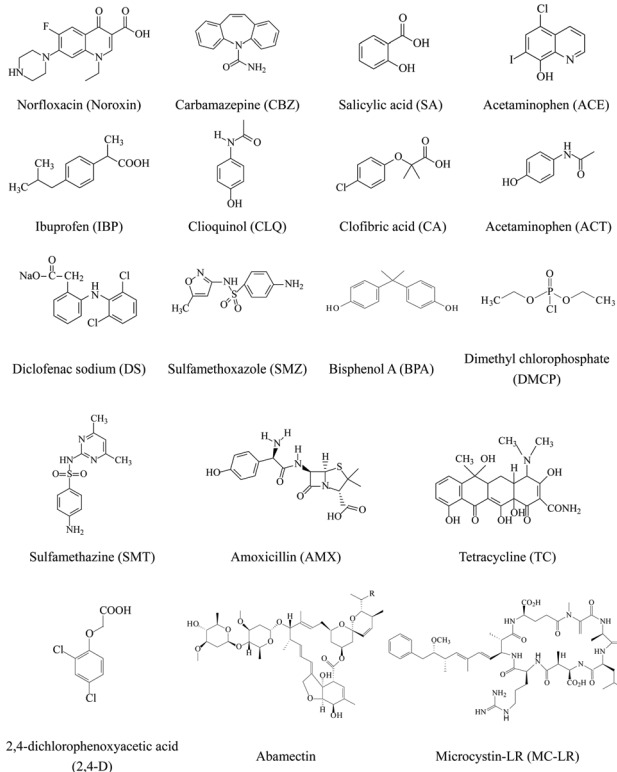
Fig. 1 Chemical structures of typical dyes, PPCPs and insecticides reported in literature studies.
