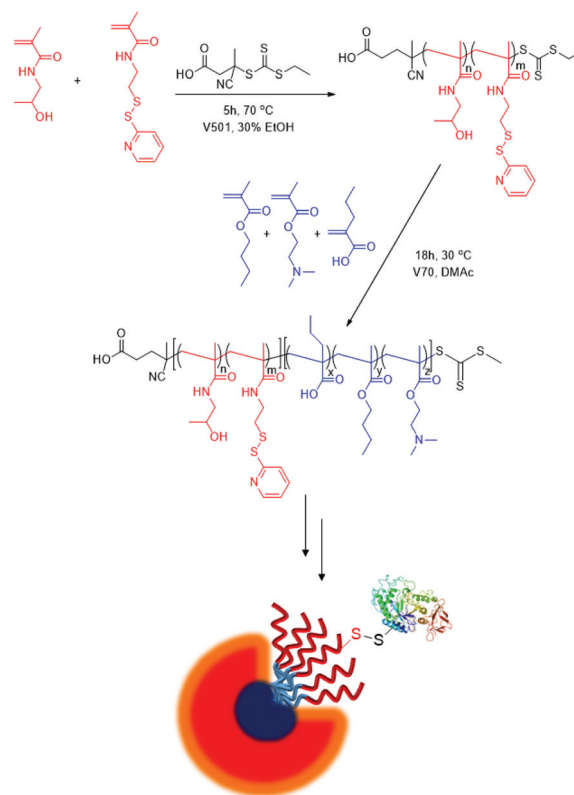
Fig. 8 Antigen conjugation on PDS-bearing pH-responsive polymers. 105 Adapted from Stayton et al. 105 with permission. Copyright © 2014 by Elsevier.
