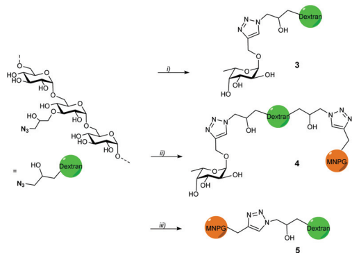
Scheme 1 Synthesis of fucose- and hybrid polymers. (i) Dextran azide, 1 , \text{CuSO}_4 , Na-CuAAC ascorbate, 100 °C, 75%, (ii) dextran azide, 1 , 2 , \text{CuSO}_4 , Na-ascorbate, 100 °C, 81%, (iii) dextran azide, 2 , \text{CuSO}_4 , Na-ascorbate, 100 °C, 51–58%.
