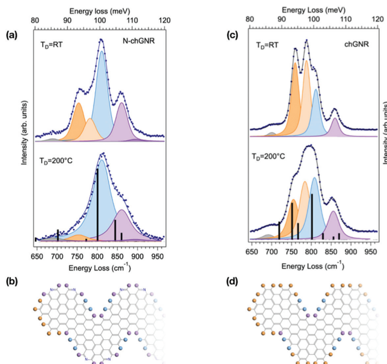
Fig. 3 Comparison between the HREEL spectra of N-doped (a) and pristine (c) chevron-type GNRs, obtained by deposition at T_D = 200 °C and at RT. The corresponding fitting components are shown as shaded curves, while calculated modes are displayed as black bars. The corresponding molecular schemes, showing the structure of the termini, are reported in (b) and (d), respectively. The top spectrum in (a) is also reported in the right panel of Fig. 1.
