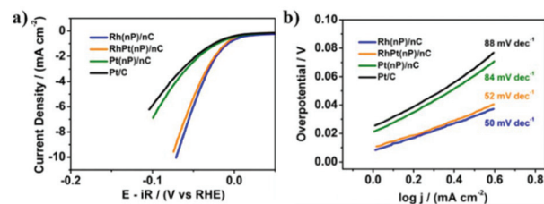
Fig. 3 HER performance of Rh(nP)/nC, RhPt(nP)/nC, Pt(nP)/nC and commercial Pt/C in 0.1 M KOH solution. (a) LSV polarization curves at a scan rate 5 \text{ mV s}^{-1} . (b) Corresponding Tafel plots. The potentials were corrected for iR drop and calibrated to RHE.
