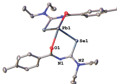
Fig. 3 Molecular structure of 1a . Thermal ellipsoids are drawn at the 50% probability level. Hydrogen atoms have been omitted for clarity.
