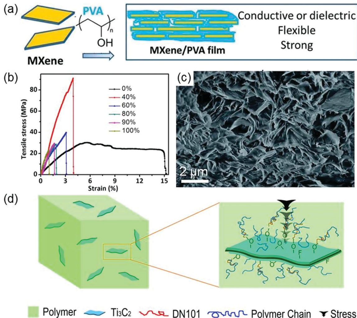
Fig. 4 (a) Schematic for the synthesis of the Ti_3C_2T_x -PVA composite. (b) Stress-strain curves for Ti_3C_2T_x -PVA films with different Ti_3C_2T_x weights. Reprinted with permission from ref. 78 Copyright (2014) PNAS. (c) SEM fracture surface morphology images of the 6 wt% Ti_3C_2T_x -PAM sample. Reprinted with permission from ref. 79 Copyright (2016) Royal Society of Chemistry. (d) Schematic representation of forces on the Ti_3C_2T_x -UHMWPE composite. Reprinted with permission from ref. 80 Copyright (2015) Elsevier.
