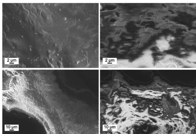
Fig. 6 SEM images of sample 7 (left) and sample 8 (right) at two different magnifications. No microcrystals can be observed on the polymer surface for both samples.
