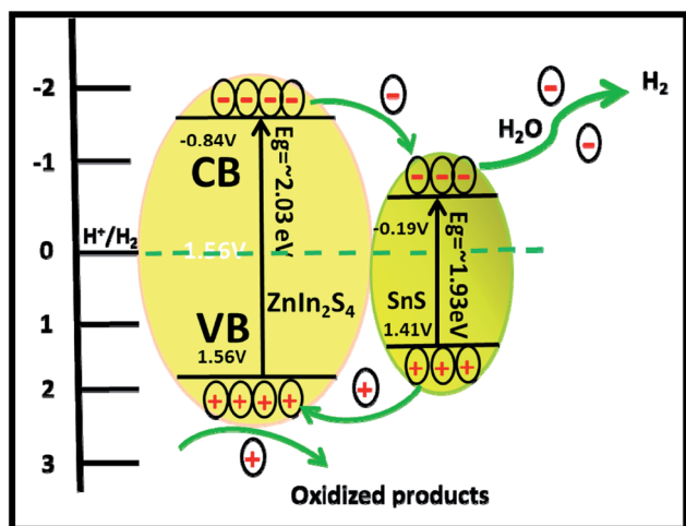
Scheme 2 Schematic of the photocatalytic mechanism of \text{SnS}@ZnIn_2S_4 heterostructures.
