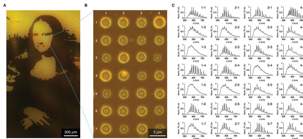
Fig. 6 Micro-hemisphere array of 1 with individual WGM fingerprints. (A) Fluorescence micrograph of a micropainting (1.6 × 2.7 mm 2 ) drawn on a quartz substrate, prepared by irradiation at \lambda = 350\text{--}390 nm for 3 min of the microarray of 1 through a patterned photomask. (B) Optical micrograph of the resultant micro-hemisphere array with a 4 × 7 matrix. (C) PL spectra of the arrayed micro-hemispheres. The labels correspond to the matrix in (B).
