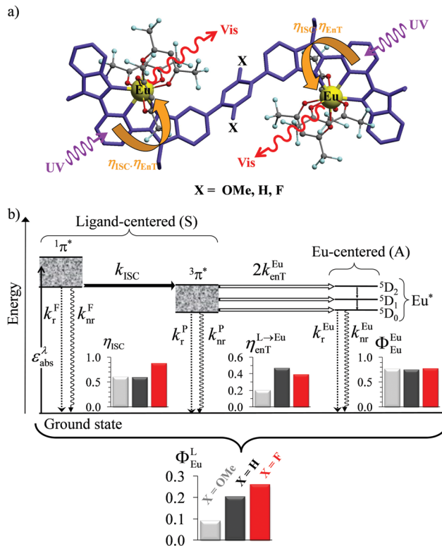
Fig. 6 (a) Molecular structures and (b) simplified Jablonski diagram for [(\text{hfac})_3\text{Eu}]_2\text{L}[(\text{hfac})_3\text{Eu}] showing the indirect ligand-centred triplet-mediated sensitization mechanism of the two \text{Eu}^{3+} activators. The photophysical processes are described by first-order rate constants: k_r^{\text{L}} = ligand fluorescence, k_{\text{nr}}^{\text{L}} = ligand internal non-radiative conversion, k_{\text{ISC}}^{\text{L}} = ligand phosphorescence, k_{\text{nr}}^{\text{L}} = non-radiative relaxation from the ligand triplet state, k_r^{\text{Eu}} = emission of \text{Eu}^* , k_{\text{nr}}^{\text{Eu}} = nonradiative decay of \text{Eu}^* , k_{\text{ISC}}^{\text{L}} = ligand intersystem crossing, and k_{\text{en.tr.}}^{\text{L} \rightarrow \text{Eu}} = ligand-to-metal energy transfer. Efficiencies of intersystem crossing ( \eta_{\text{ISC}} ), of energy transfer ( \eta_{\text{en.tr.}}^{\text{L} \rightarrow \text{Eu}} ), of intrinsic quantum yield ( \Phi_{\text{Eu}}^{\text{L}} ), and global quantum yield ( \Phi_{\text{Eu}}^{\text{L}} ) characterize the antenna effect (solid-state, 293 K). Adapted from ref. 17b.
