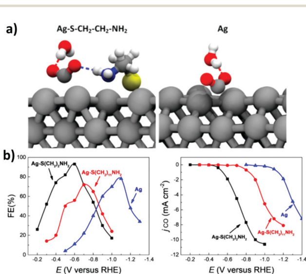
Fig. 31 (a) Chemisorbed \text{CO}_2 on cysteamine-functionalized (left) and cysteamine-free (right) Ag(111) surface. Only the water molecules directly forming hydrogen bond (slashed line) are shown. The colors are: Ag in silver, C in gray, O in red, N in blue, S in yellow, and H in white. (b) Influence of the alkyl chain length on \text{CO}_2 RR in terms of \text{FE}_{\text{CO}} (left) or j_{\text{CO}} (right) vs. potential. Reproduced with permission from ref. 419. Copyright 2018 American Chemical Society.
