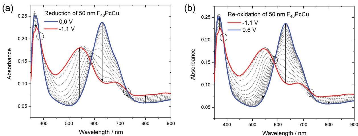
Fig. 9 Optical absorption spectra of a 50 nm thin film of F_{40}PcCu measured during cyclic voltammetry at 0.05 \text{ V s}^{-1} upon (a) reduction and (b) re-oxidation of the film. The isosbestic points and ranges are marked by circles.
