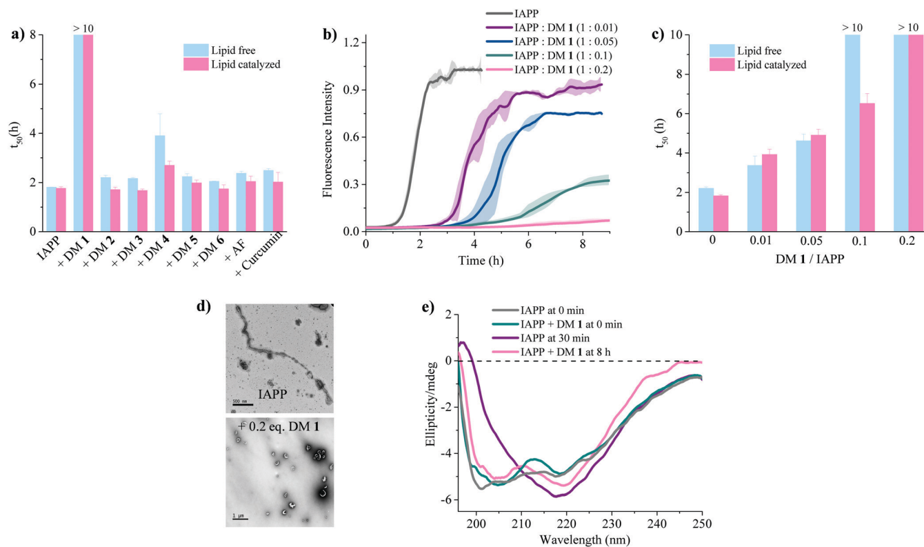
Fig. 3 Anti-amyloidogenic activity of DM 1 against IAPP self-assembly. (a) Comparison of t_{50} 's of IAPP aggregation in presence of the indicated ligands at a stoichiometric ratio of 1 : 0.2 (IAPP : ligand). Lipid free condition: IAPP = 25 \mu\text{M} in phosphate buffer (50 mM NaPi, 150 mM KCl, pH 7.4) [ThT] = 12.5 \mu\text{M} ; lipid catalysed condition: IAPP = 15 \mu\text{M} in phosphate buffer (50 mM NaPi, 150 mM KCl, pH 7.4) including LUVs (DOPG : DOPC, 3 : 7, 750 \mu\text{M} , d = 100 nm). [ThT] = 7.5 \mu\text{M} . (b) ThT-based kinetic profile of lipid catalysed IAPP aggregation in the absence and presence of DM 1 at the indicated sub-stoichiometric ratios. Solid curves represent the average of three independent trials while the shaded regions represent the standard deviations of those measurements. (c) Statistical analysis of t_{50} 's of IAPP aggregation in the presence of different concentrations of DM 1 . (d) TEM images of 15 \mu\text{M} IAPP after 2 h (top) and in presence of DM 1 (3 \mu\text{M} ) after 8 h (bottom) under lipid catalysed condition. (e) Circular dichroism spectra of 15 \mu\text{M} IAPP in the absence (gray and purple curves) and presence (green and pink curves) of DM 1 in lipid catalysed conditions at different time intervals depicted in the figure.
