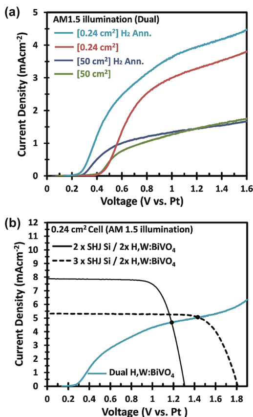
Fig. 9 (a) J - V curves comparing the effects of hydrogen annealing on the small and large area dual- \text{CoP}_i/\text{W}:\text{BiVO}_4 photoanodes in 0.1 M \text{KP}_i (small area) or 2.0 M \text{KP}_i (large area) buffer. Large area samples are with Ni lines. (b) J - V curves of a small area 2 SHJ PV (black line) and the 3 SHJ PV (dashed black line) with dual- \text{CoP}_i/\text{H,W}:\text{BiVO}_4 photoanodes as the front windows, and the small area dual- \text{CoP}_i/\text{H,W}:\text{BiVO}_4 photoanode, measured in 0.1 M \text{KP}_i buffer.
