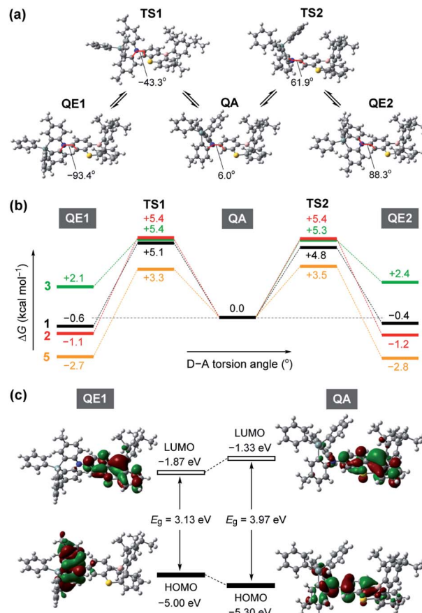
Fig. 3 (a) Molecular geometrical changes in 1 along the interconversion between its quasi-equatorial (QE) and quasi-axial (QA) conformers through the transition states (TS). (b) Energy profiles for the interconversion processes of 1–3 and 5 in their ground states at 298 K and 1 atm, calculated at the B3LYP/6-31G(d) level of theory. (c) Spatial distribution of the frontier orbitals (HOMOs and LUMOs) for the ground-state QE and QA conformers of 1.
