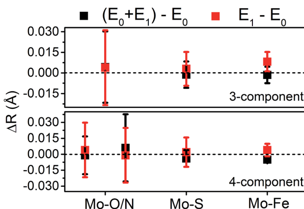
Fig. 5 Comparison of variation in determined bond distances from Mo K-edge EXAFS. Changes in distances are calculated by subtraction of the fit E_0 distances from those of the turnover ( E_0 + E_1 ) and E_1 fits. Error bars are reported on a 95% confidence interval.
