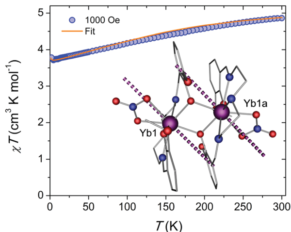
Fig. 1 Temperature dependence of the \chi T product at 1000 Oe (blue spheres), and comparison with the calculated magnetic susceptibility assuming J = 0.005 \text{ cm}^{-1} (solid orange line). The inset displays the molecular structure of the \{\text{Yb}_2\} complex along with the orientation of the main magnetic axis in the ground state of the \text{Yb}^{\text{III}} ions as shown in the purple dashed lines. Colour code: purple (Yb), red (O), blue (N); while all unfilled grey vertices represent carbon atoms.
