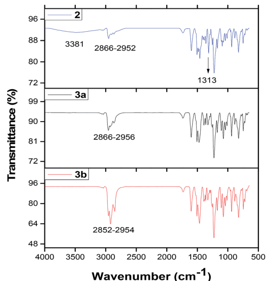
Fig. 1 FTIR spectra of complexes 2 , 39 3a and 3b .
