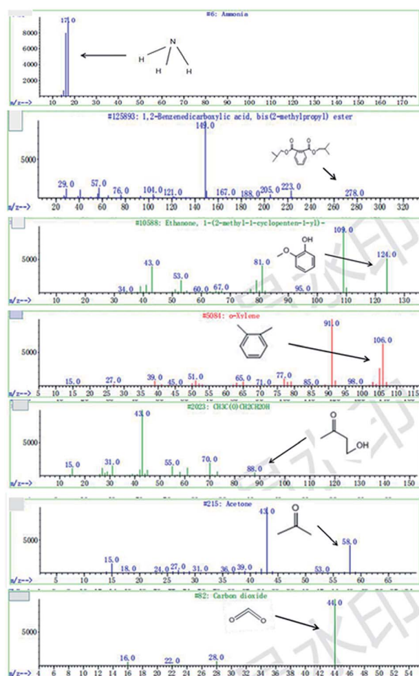
Fig. 10 GC-MS analysis of degradation products about Disperse Red 3B.
