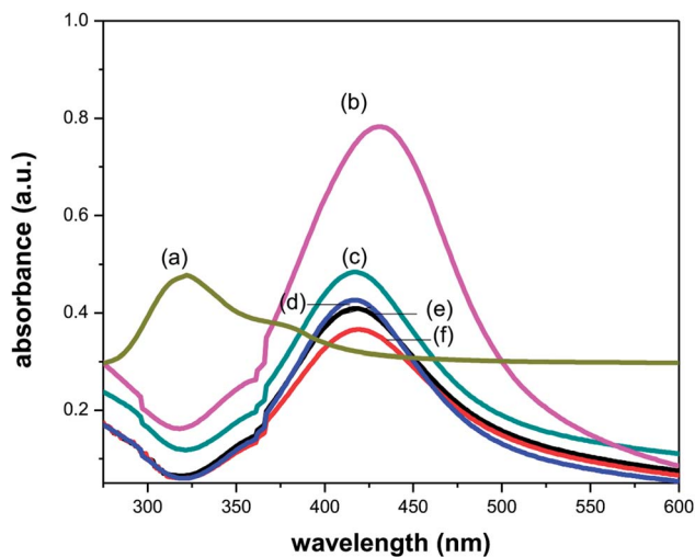
Fig. 3 UV-vis absorption spectra of (a) amikacin, (b) PVP-AgNPs, (c–f) Amk@PVP-AgNPs at concentration 0.05 , 0.1 , 0.3 and 0.5 \text{ mM} respectively.
