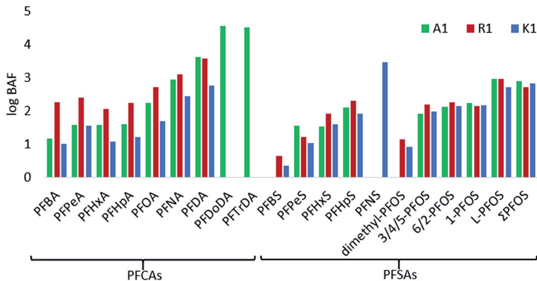
Fig. 4 The logarithmic bioaccumulation factor (BAF) on a wet weight basis ( L\ kg^{-1} ) of target PFCAs and PFSA (including four branched PFOS isomers, linear PFOS and \Sigma PFOS) for sites A1, R1 and K1. The BAFs could not be determined for some PFASs and sites due to values below MDL.
